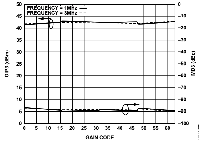
Figure 55. OIP3 on Low Frequency, 2 V p-p Composite
